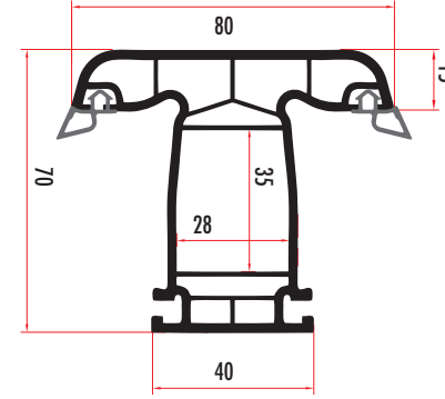
YAK71531 70 MM ORTA KAYIT MULLION PROFILE YAK71532 (RENKLİ/COLORED)
