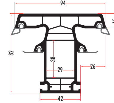
QUA8231 82 MM 6 ODACIKLI ORTA KAYIT MULLION PROFILE QUA8232 (RENKLİ/COLORED)
