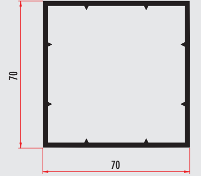
YARK70701 70 X 70 KUTU PROFİLİ 70 X 70 BOX PROFILE YARK70702 (RENKLİ/COLORED)
