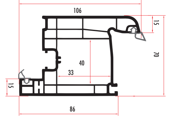
YAK71551 70 MM KAPI KANAT DOOR SASH PROFILE YAK71552 (RENKLİ/COLORED)
