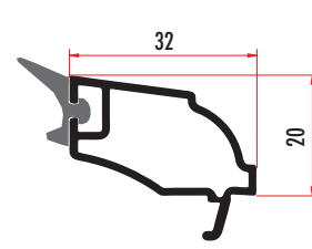
CAM5411 10 MM DEKORATİF TEK CAM ÇİTASI 10 MM DECORATIVE GLAZING BEAD CAM5412 (RENKLİ/COLORED)
