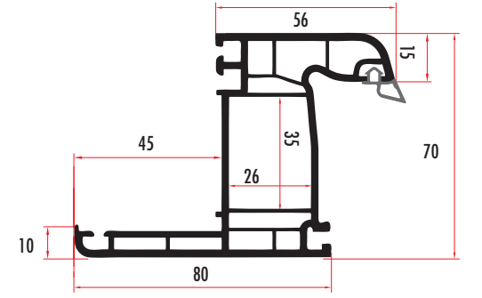
YAK71521 70 MM PERVAZLI KASA FRAME PROFILE WITH BORDER YAK71522 (RENKLİ/COLORED)
