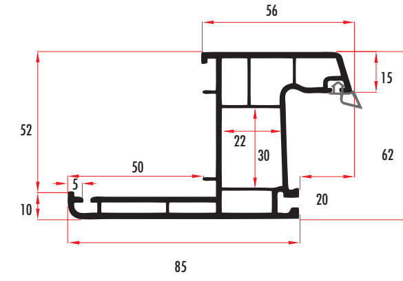
ENR62321 62 MM 3 ODACIKLI PERVAZLI KASA FRAME PROFILE WITH BORDER ENR62322 (RENKLİ/COLORED)
