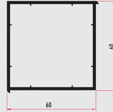
YARK60601 60 X 60 KUTU PROFİLİ 60 X 60 BOX PROFILE YARK60602 (RENKLİ/COLORED)
