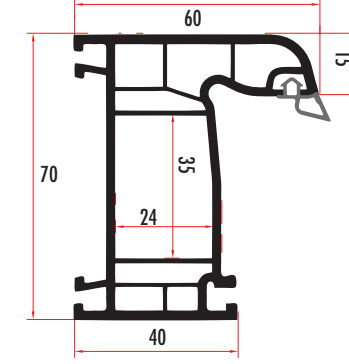
YAK71511 70 MM KASA / FRAME PROFILE YAK71512 (RENKLİ/COLORED)
