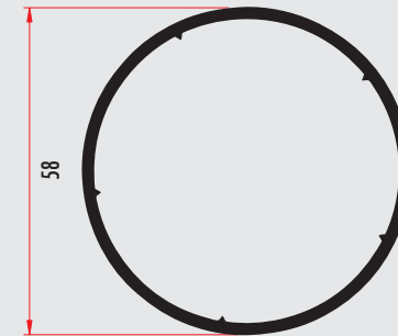
YARA41 BORU PROFİLİ PIPE PROFILE YARA42 (RENKLİ/COLORED)
