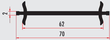
YARI701 70 MM FIX I BAĞ PROFİLİ CONNECTION PROFILE FOR 70 MM SERİE YARI702 (RENKLİ/COLORED)
