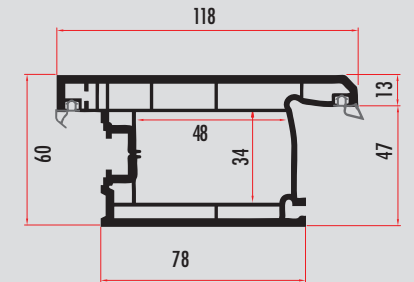
TRU60361 60 MM 3 ODACIKLI DIŞA AÇILIR KAPI KANAT OUTWARD OPENING DOOR SASH PROFILE TRU60362 (RENKLİ/COLORED)
