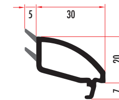
20 MM OVAL SERİ ÇİFT CAM ÇİTASI 20 MM DOUBLE GLAZING BEAD CAM7122 (RENKLİ/COLORED)
