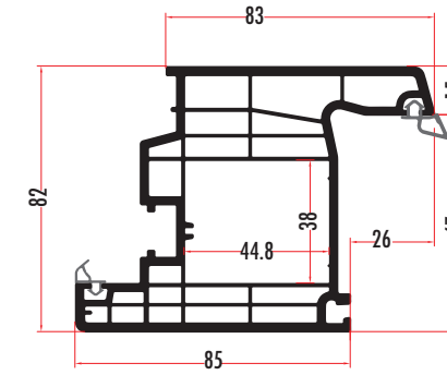
QUA8251 82 MM 6 ODACIKLI KAPI KANAT DOOR SASH PROFILE QUA8252 (RENKLİ/COLORED)
