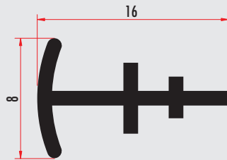
YARI62B1 FIX I BİRLEŞİM PROFİLİ CONNECTION PROFILE FOR 62 MM SERİE YARI62B2 (RENKLİ/COLORED)
