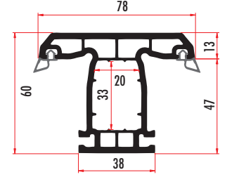
TRU60331 60 MM. 3 ODACIKLI ORTA KAYIT MULLION PROFILE TRU60332 (RENKLİ/COLORED)
