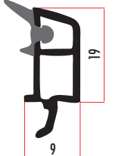
CAM5431 32 MM ÜÇ CAM ÇİTASI 32 MM TRIPLE GLAZING BEAD CAM5432 (RENKLİ/COLORED)
