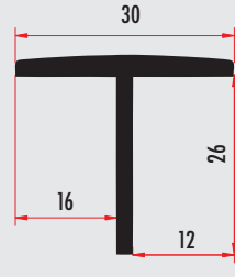
YARTK1 DAR T KAPAMA PROFİLİ T CLOSER PROFILE YARTK2 (RENKLİ/COLORED)
