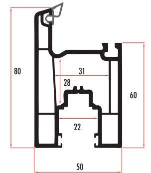
SIT7641 SÜRME KANAT /SLIDING SASH PROFILE SIT7642 (RENKLİ/COLORED)
