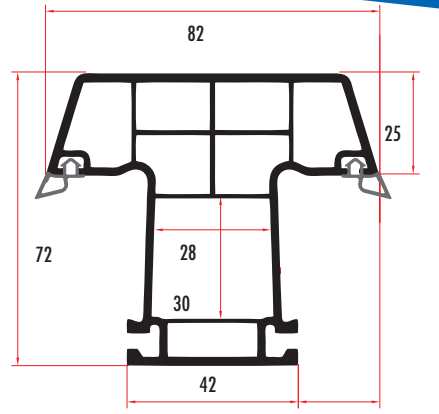
KUV 72421 72 MM 3 ODACIKLI ORTA KAYIT MULLION PROFILE KUV 72422 (RENKLİ/COLORED)
