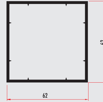
YARK62621 62X62 KUTU PROFİLİ 62 X 62 BOX PROFILE YARK62622 (RENKLİ/COLORED)
