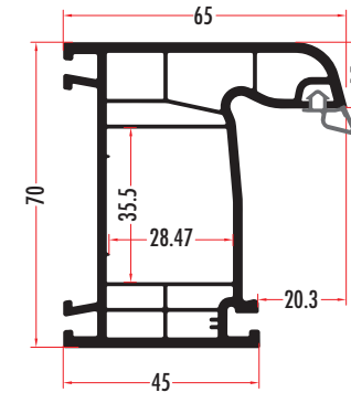
YAK72511 70 MM KASA / FRAME PROFILE YAK72512 (RENKLİ/COLORED)
