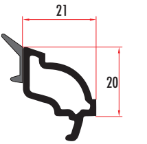
CAM6021 20 MM DEKORATİF ÇİFT CAM ÇİTASI 20 MM DECORATIVE DOUBLE GLAZING BEAD CAM6022 (RENKLİ/COLORED)
