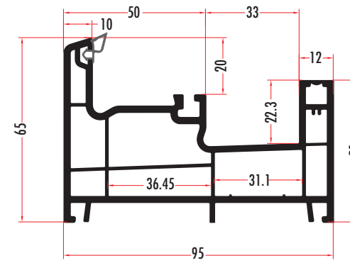
SIT7681 76 MM TEK RAYLI SÜRME KASA SINGLE RAILED SLIDING FRAME PROFILE SIT7682 (RENKLİ/COLORED)
