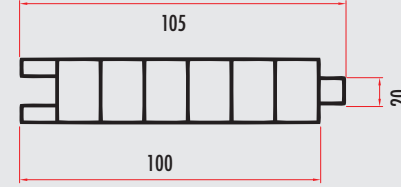
YARP11 PANEL PROFİLİ PANEL PROFILE YARP12 (RENKLİ/COLORED)
