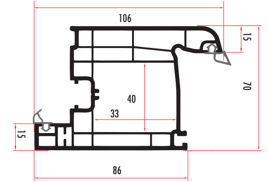
LAP71551 70 MM KAPI KANAT DOOR SASH PROFILE LAP71552 (RENKLİ/COLORED)
