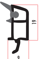
CAM5431 32 MM ÜÇ CAM ÇİTASI 32 MM TRIPLE GLAZING BEAD CAM5432 (RENKLİ/COLORED)
