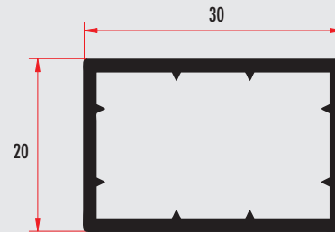
ZIR8661 TEK RAYLI SÜRME KASA YAN KAPATMA PROFİLİ ADOPTER FOR SINGLE RAILED SLIDING FRAME PROFILE ZIR8662 (RENKLİ/COLORED)
