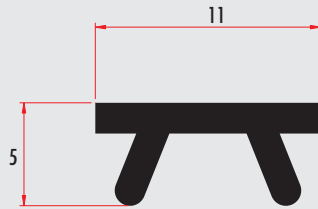
ZIR8651 SÜRME SERİ RAY KAPATMA PROFİLİ RAIL CLOSER ZIR8652 (RENKLİ/COLORED)
