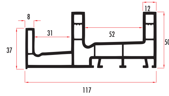
SIT7621 SİNEKLİKLİ SÜRME KASA DOUBLE RAILED SLIDING FRAME PROFILE WITH FLY SCREEN SIT7622 (RENKLİ/COLORED)
