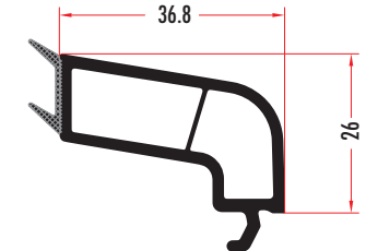
QUA8221 24 MM ÇİFT CAM ÇİTASI 24 MM DOUBLE GLAZING BEAD QUA8222 (RENKLİ/COLORED)
