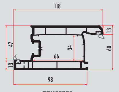
TRU60351 60 MM 3 ODACIKLI KAPI KANAT DOOR SASH PROFILE TRU60352 (RENKLİ/COLORED)
