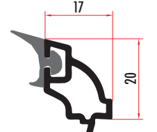
CAM5421 24 MM DEKORATİF ÇİFT CAM ÇİTASI 24 MM DECORATIVE GLAZING BEAD CAM5422 (RENKLİ/COLORED)
