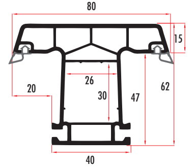
PEG62431 62 MM 4 ODACIKLI ORTA KAYIT / MULLION PROFILE PEG62432 (RENKLİ/COLORED)
