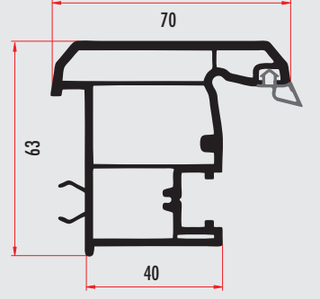
YARP21 PLUS HAREKETLİ ORTA KAYIT PROFİLİ PLUS MOVABLE MULLION PROFILE YARP22 (RENKLİ/COLORED)
