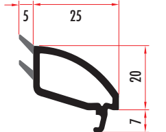
CAM7131 24 MM OVAL SERİ ÇİFT CAM ÇİTASI 24 MM DOUBLE GLAZING BEAD CAM7132 (RENKLİ/COLORED)
