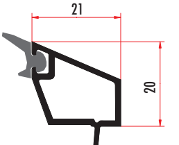
CAM6041 20 MM DÜZ ÇİFT CAM ÇİTASI 20 MM DOUBLE GLAZING BEAD CAM6042 (RENKLİ/COLORED)
