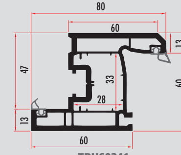
TRU60341 60 MM. 3 ODACIKLI PENCERE KANAT WINDOW SASH PROFILE TRU60342 (RENKLİ/COLORED)
