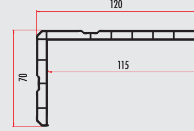
YARP31 70 X 120 PERVAZ PROFİLİ 70 X 120 BORDER PROFILE YARP32 (RENKLİ/COLORED)
