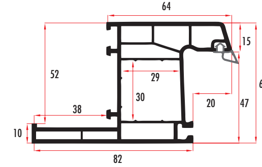
PEG62421 62 MM 4 ODACIKLI PERVAZLI KASA / FRAME PROFILE WITH BORDER PEG62422 (RENKLİ/COLORED)
