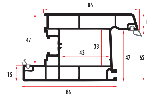
PEG62451 62 MM 3 ODACIKLI KAPI KANAT / DOOR SASH PROFILE PEG62452 (RENKLİ/COLORED)
