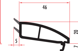
4 MM OVAL SERİ TEK CAM ÇİTASI 4 MM SINGLE GLAZING BEAD CAM7112 (RENKLİ/COLORED)
