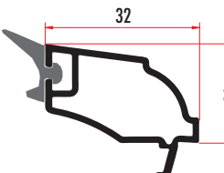
CAM5411 10 MM DEKORATİF TEK CAM ÇİTASI 10 MM DECORATIVE GLAZING BEAD CAM5412 (RENKLİ/COLORED)
