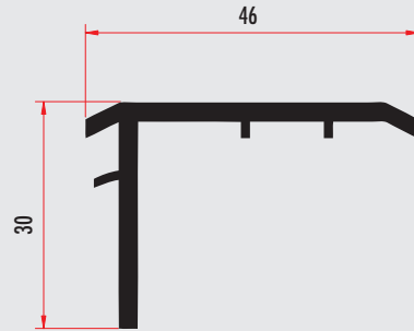
YARI1K1 L ADAPTOR PROFİLİ L ADAPTER PROFILE YARI1K2 (RENKLİ/COLORED)
