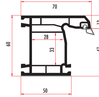
ATL60411 60 MM 4 ODACIKLI SUPER KASA SUPER FRAME PROFILE ATL60412 (RENKLİ/COLORED)
