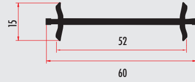
YARI601 60 MM FIX I BAĞ PROFİLİ CONNECTION PROFILE FOR 60 MM SERİE YARI602 (RENKLİ/COLORED)
