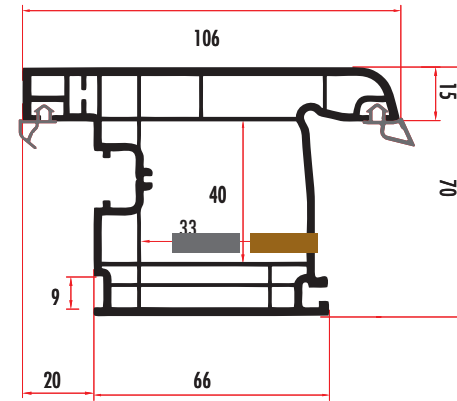
YAK71561 70 MM DIŞA AÇILIR KAPI KANAT OUTWARD OPENING DOOR SASH PROFILE YAK71562 (RENKLİ/COLORED)
