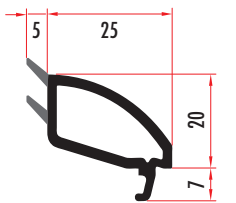
24 MM OVAL SERİ ÇİFT CAM ÇİTASI 24 MM DOUBLE GLAZING BEAD CAM7132 (RENKLİ/COLORED)
