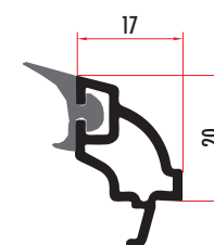
CAM5421 24 MM DEKORATİF ÇİFT CAM ÇİTASI 24 MM DECORATIVE GLAZING BEAD CAM5422 (RENKLİ/COLORED)
